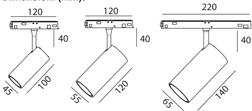
TS03/S45/BI/CO
